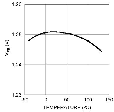
Figure 8. Feedback Voltage vs. Temperature
